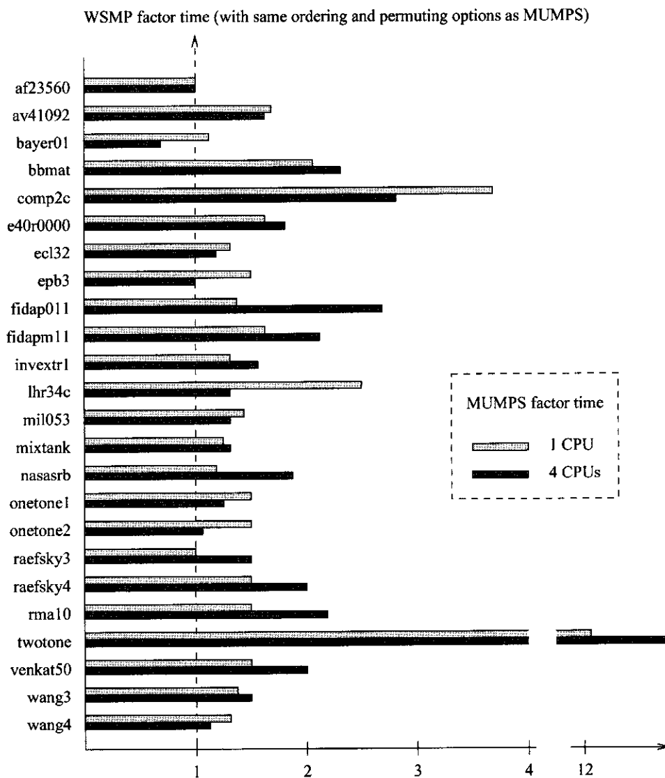
Fig. 2. Ratios of the factorization time of MUMPS to that of WSMP run with the same ordering and row-permutation option as MUMPS. This graph enables a fair comparison of the LU factorization components of the two packages.
