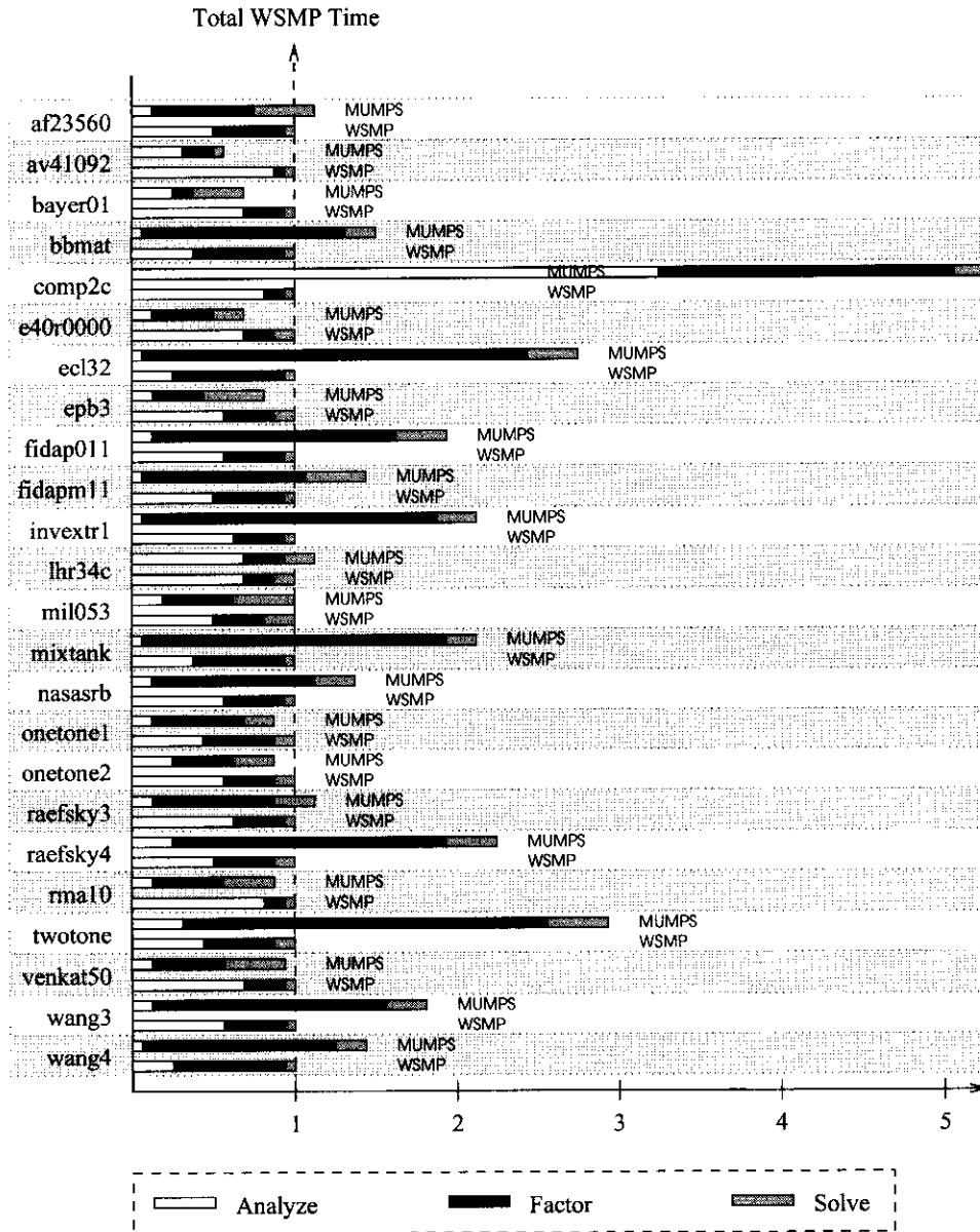
Fig. 5. A comparison of the total time taken by WSMP and MUMPS to solve a system of equations once on four CPUs of an RS6000 model 270. All times are normalized with respect to the time taken by WSMP. Furthermore, the time spent by both packages in the Analysis, Factorization, and Solve (including iterative refinement) phases is denoted by regions with different shades.
