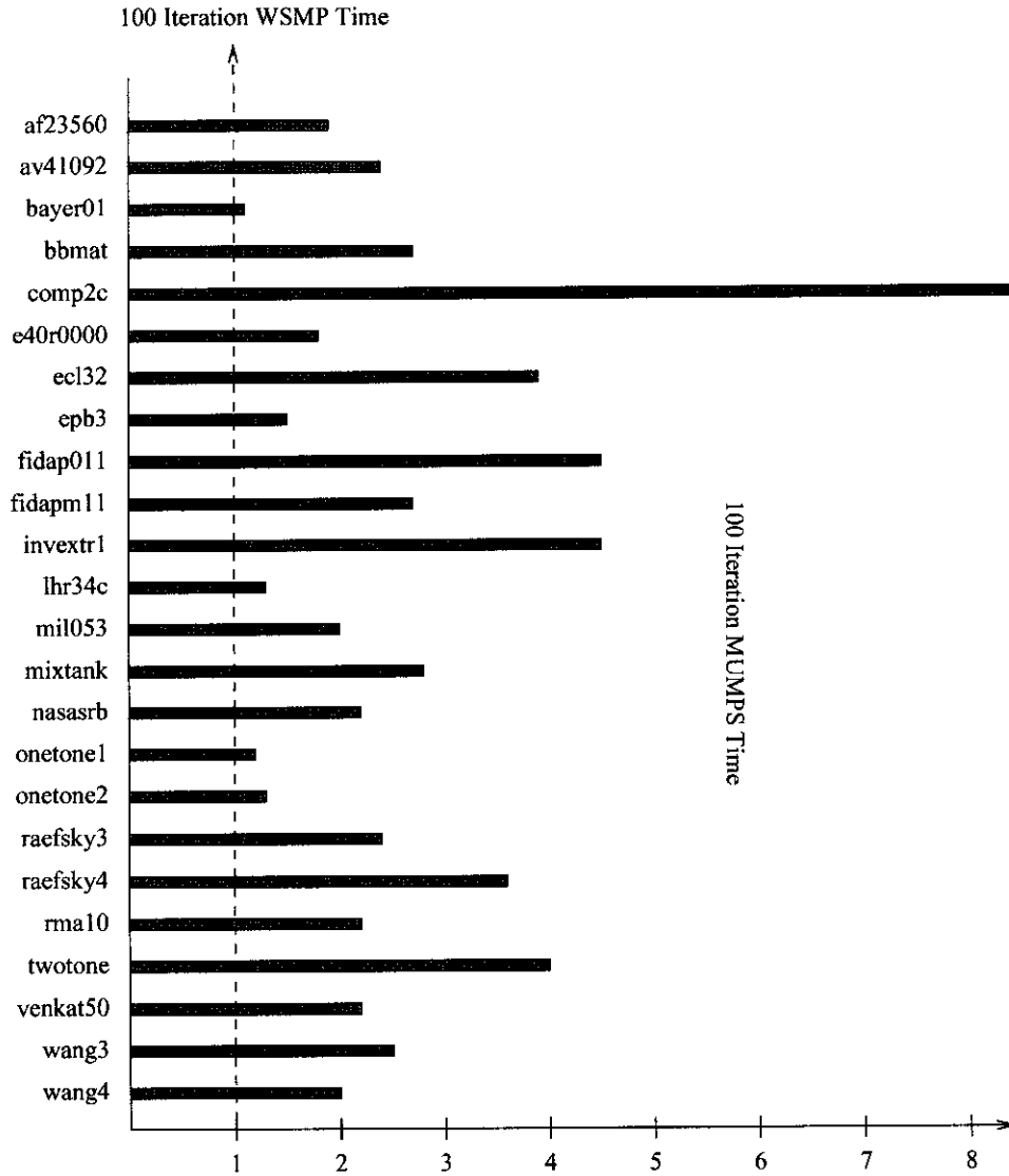
Fig. 6. A comparison of the total time taken by WSMP and MUMPS to solve 100 sparse linear systems with the same nonzero pattern and evolving coefficient values on a 4-CPU RS6000 model 270.
