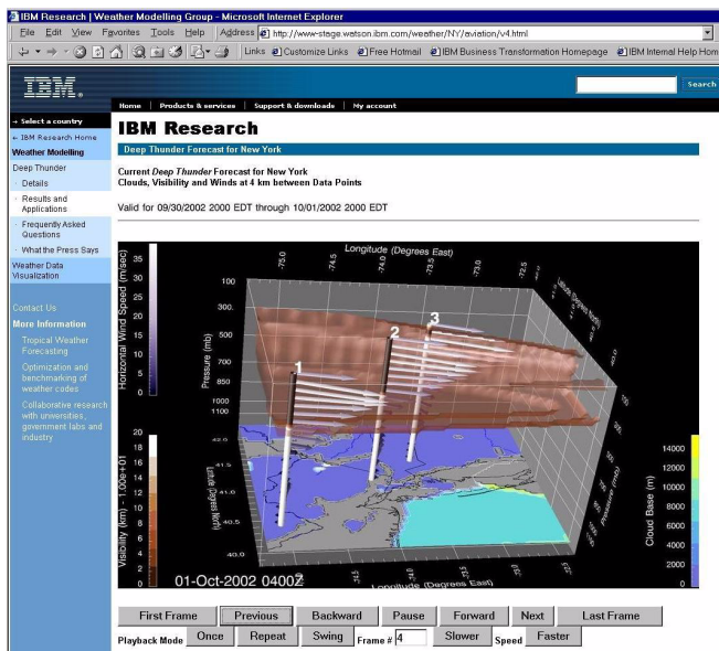
Figure 7. Animation of Cloud/Visibility Products.
