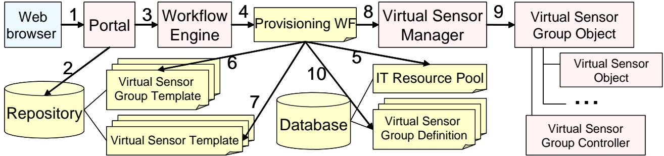
Figure 6. Provisioning Flow
