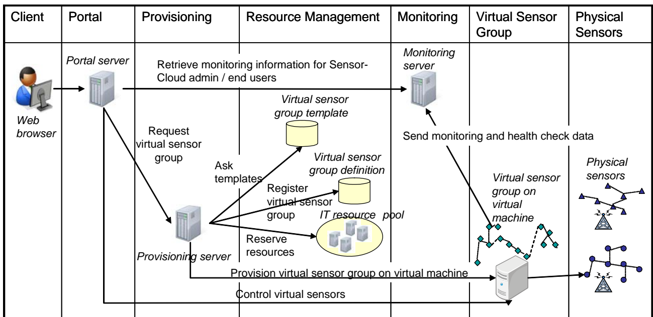
Figure 4. System Architecture of Sensor Cloud Infrastructure
