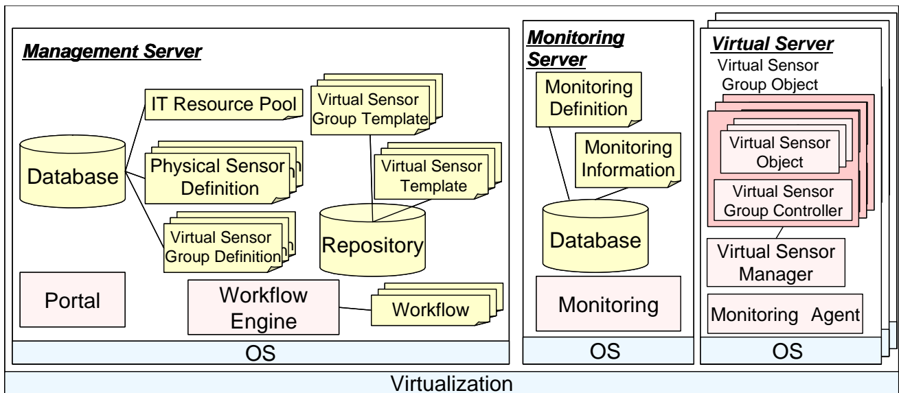
Figure 5. Prototype of Sensor Cloud Infrastructure
