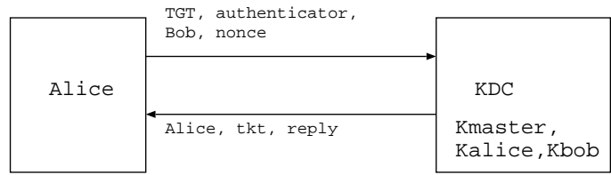
Figure 3: original TGS_REQ processing in Kerberos V5
