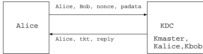
Figure 1: original AS_REQ processing in Kerberos V5
