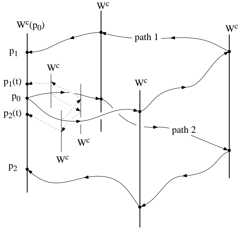
FIGURE 5. A Brin quadrilateral in which the arrows indicate the orientations of the two paths.
