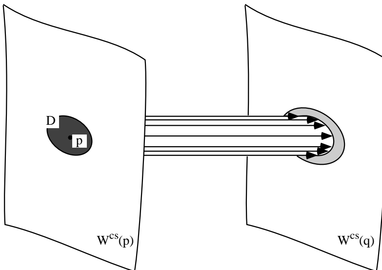
FIGURE 2. Unit holonomy along the strong unstable foliation.
