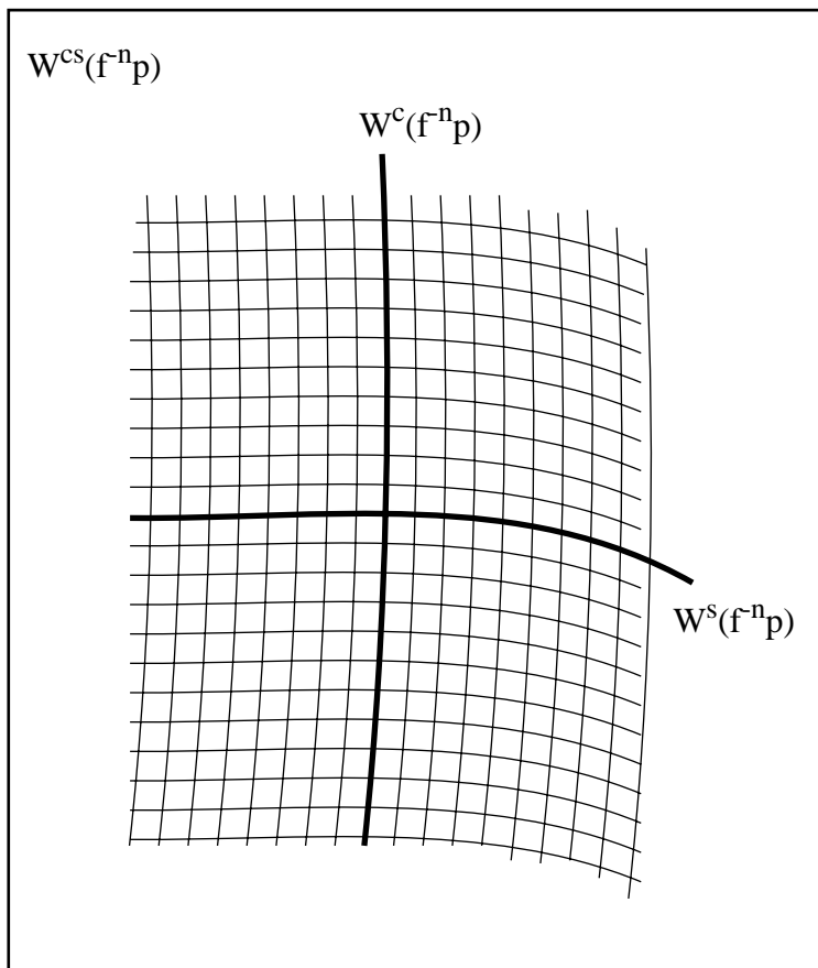
FIGURE 3. The center-stable julienne at the point f^{-n}(p) .
