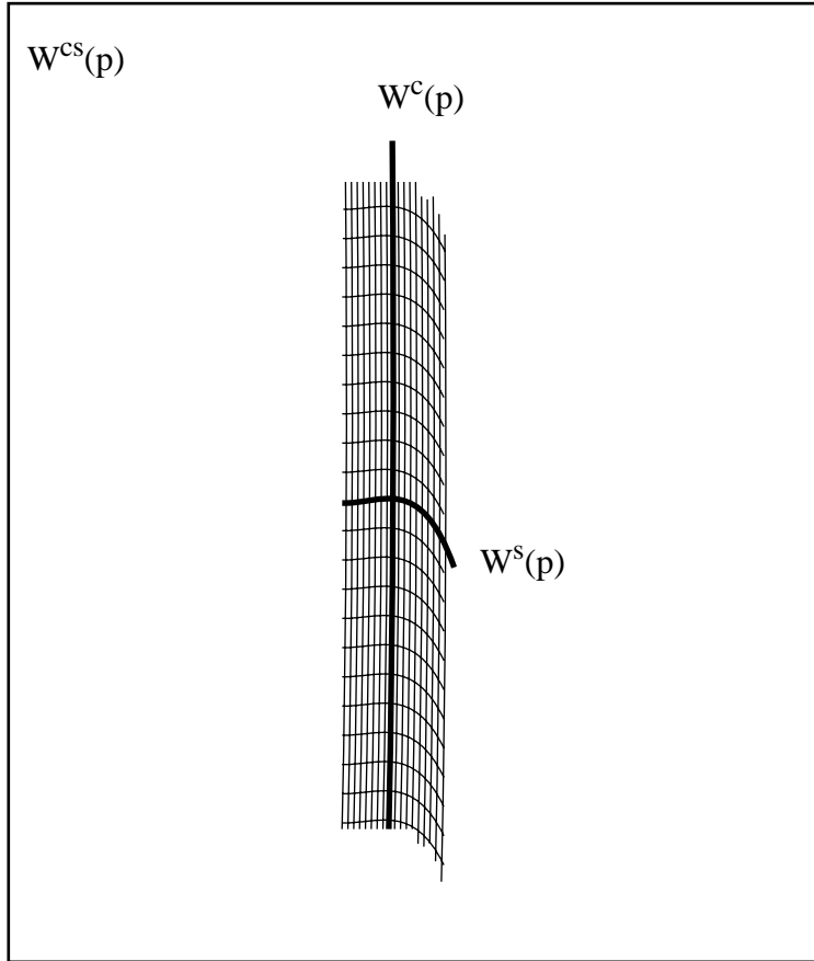
FIGURE 4. The center-stable julienne at the point p .
