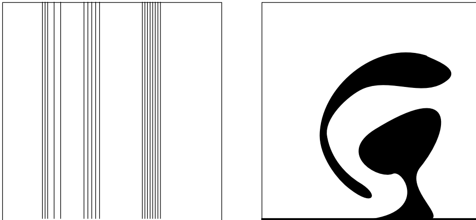
FIGURE 1. Sets in the the Borel subalgebras \mathcal{A} and \mathcal{C} .
