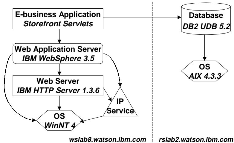
Figure 1: Simplified application dependency graph of an e-business system
