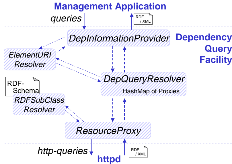
Figure 6: Components and information flows
