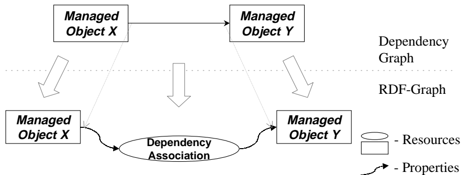
Figure 3: Mapping a dependency to RDF
