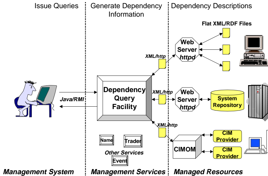
Figure 2: Architecture of our Dependency System
