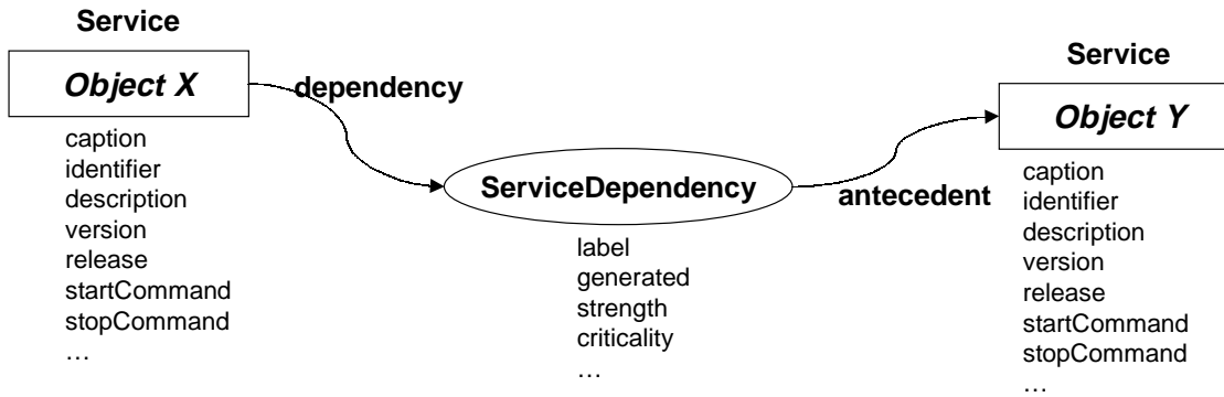
Figure 4: Elements of a dependency description in RDF
