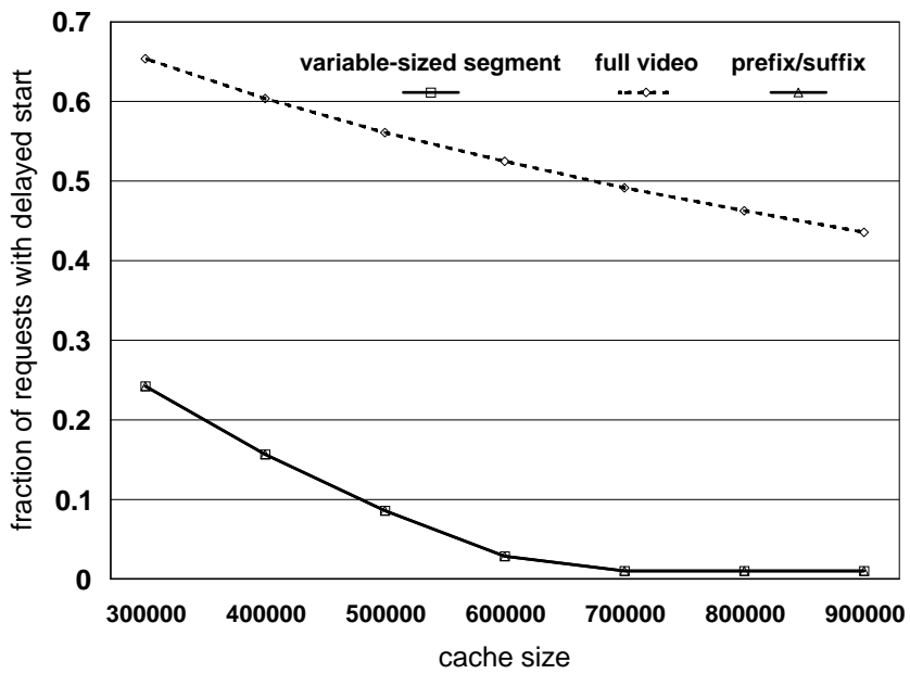
Figure 6: The impact of cache size on delayed start.
