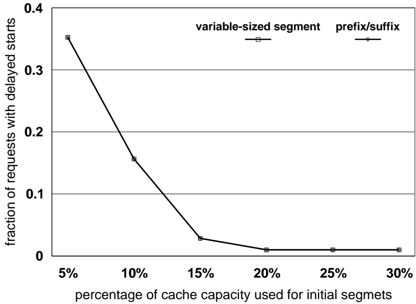
Figure 13: The impact of cache capacity used for initial segments on delayed start.
