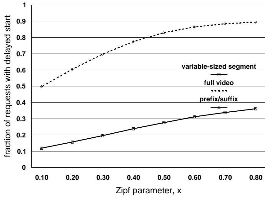
Figure 8: The impact of skew in video popularity on delayed start.
