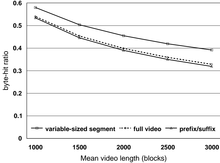
Figure 10: The impact of video length.
