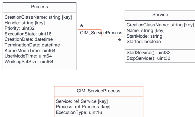
Fig. 2: The CIM_ServiceProcess association
