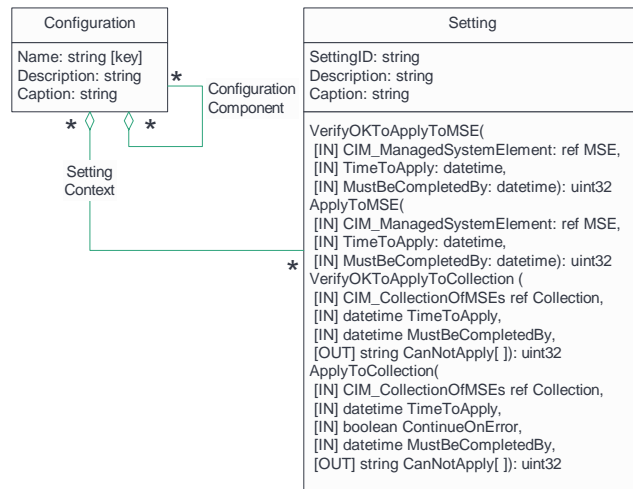
Fig. 5: CIM_Setting and CIM_Configuration (before changes)
