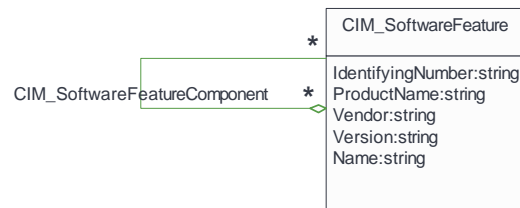
Fig. 3: CIM_SoftwareFeatureComponent
