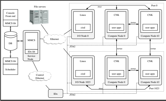
Fig. 2. Blue Gene/L system software
