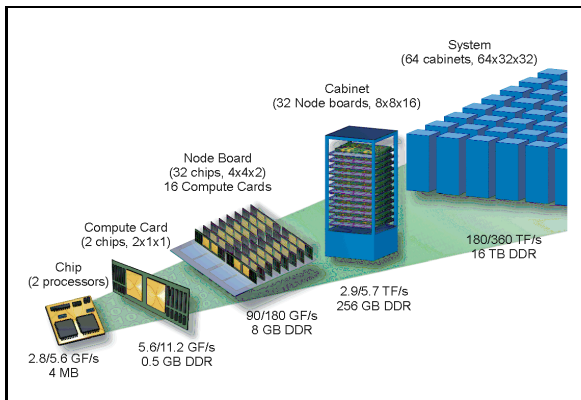
Fig. 1. High-level organization of Blue Gene/L
