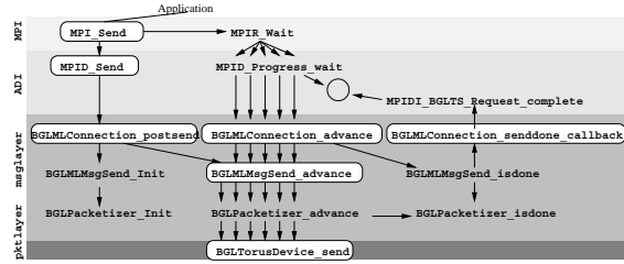
Fig. 6. The callgraph of an MPI_Send() call
