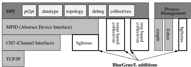
Fig. 4. The Blue Gene/L MPI roadmap
