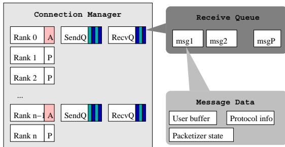
Fig. 3. The message layer architecture
