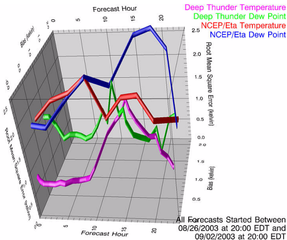
Figure 6. Example Verification Visualization.
