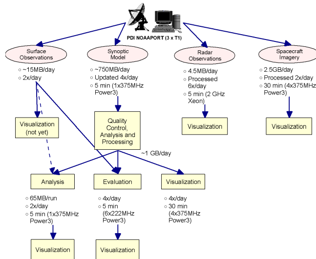
Figure 1. Pre-Processing Procedural and Data Flow.
