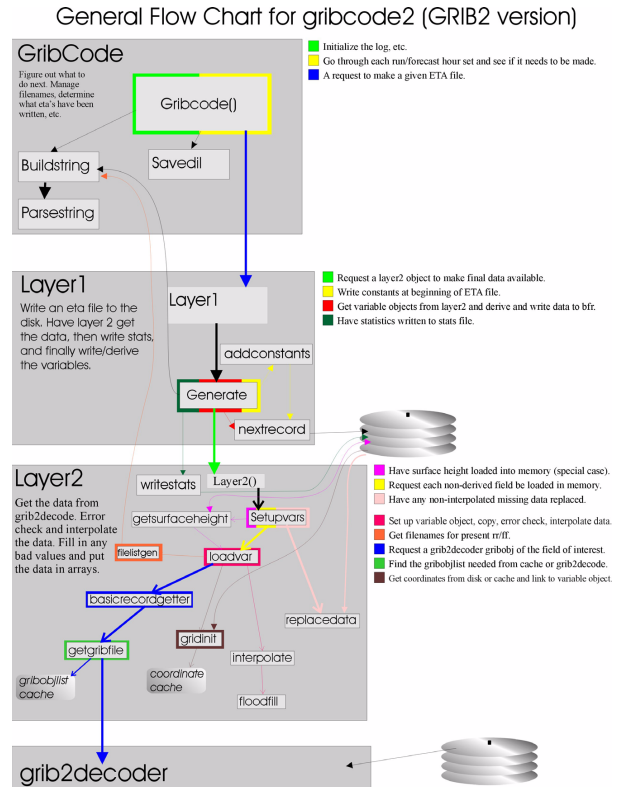
Figure 3. GriB-2 Processing Procedural and Data Flow.
