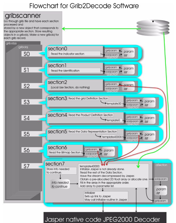
Figure 4. GriB-2 Decoding Process.
