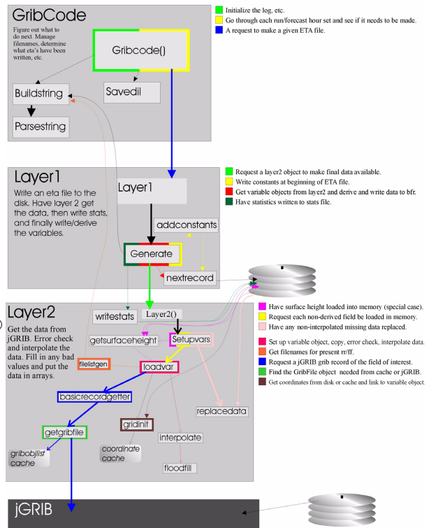
Figure 2. GriB-1 Processing Procedural and Data Flow.
