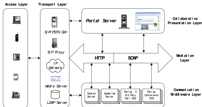
Fig. 3. Rich Media Collaborative Workplace Architecture
