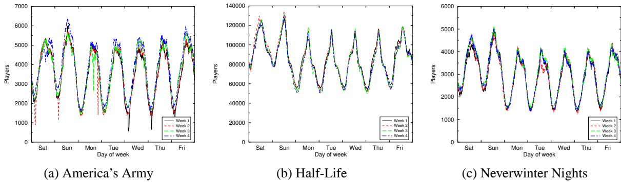
Figure 7: Player load for three popular games over a 4-week period
