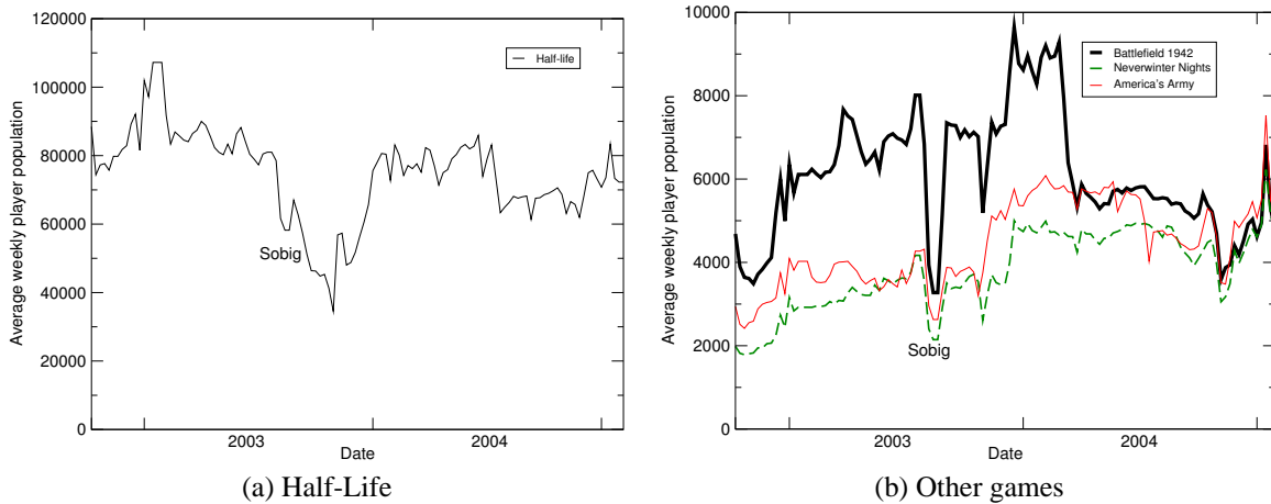
Figure 10: Population trends for Half-life and other games with an averaging window of one week
