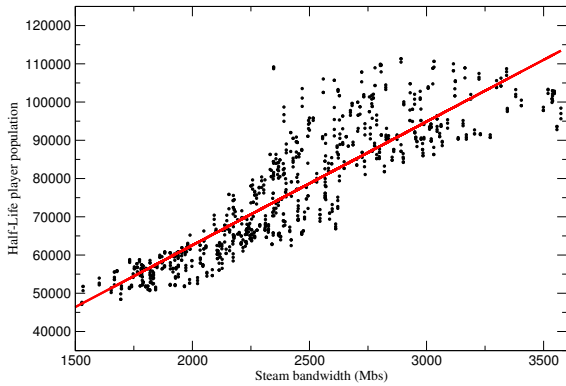
Figure 15: Half-Life player population versus Steam CDN usage
