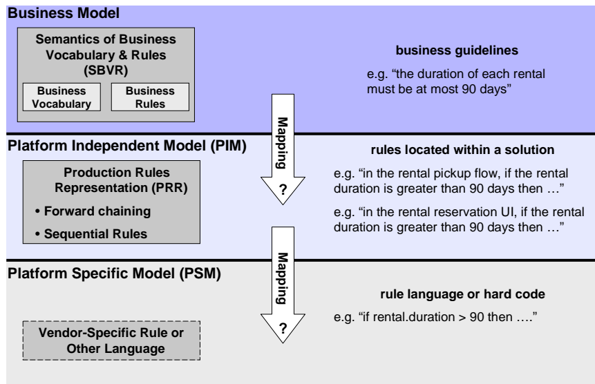
Fig. 2. Rules in the MDA Layers
