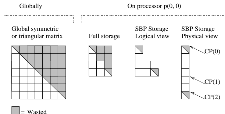
Fig. 3. Illustration of how a 7 \times 7 block global matrix is laid out on a 2 \times 3 mesh in SBP format and addressed with its column pointer (CP) array. The full size of the global matrix is 7NB \times 7NB .
