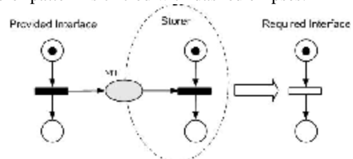
(a) Extra sending message scenario
