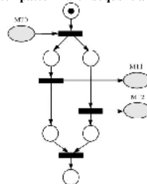
(b) Splitter pattern with parallel structure
