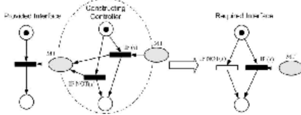
(b) Missing condition of receiving messages scenario
