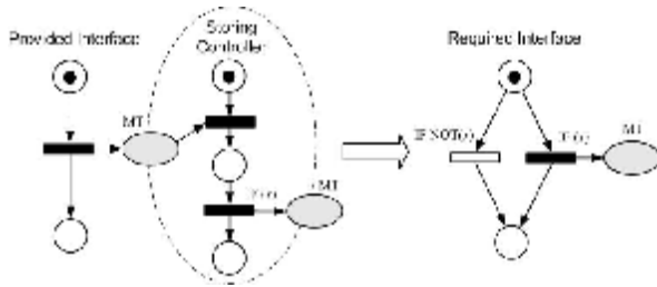
(b) Missing condition of sending messages scenario Figure 9. Scenarios of using Storing Controller pattern
