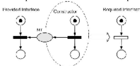
(a) Extra receiving message scenario
