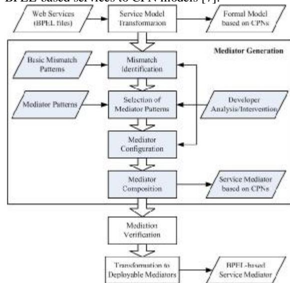
Figure 2. Solution approach to protocol mediation
