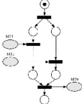
(b) Merger pattern with parallel structure
