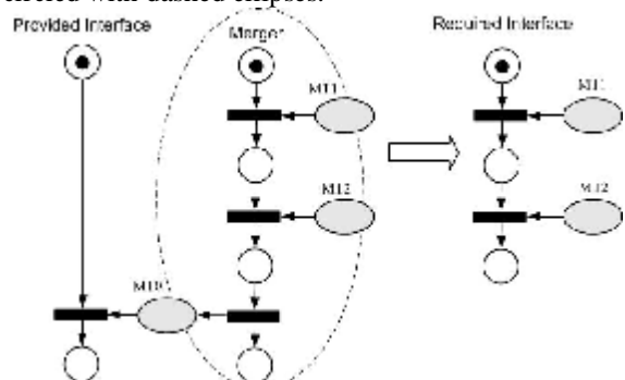
(a) Splitting receiving messages scenario
