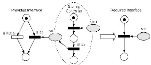
(a) Extra condition of receiving messages scenario
