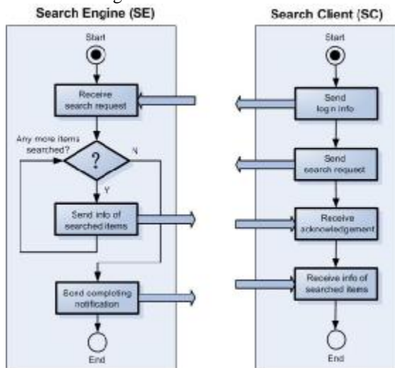
Figure 1. A motivating example of service composition with protocol mismatches
