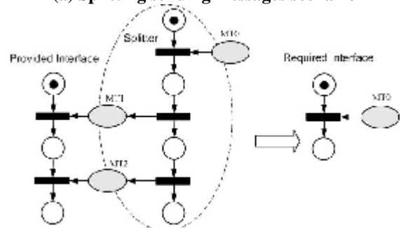
(a) Splitting sending messages scenario
