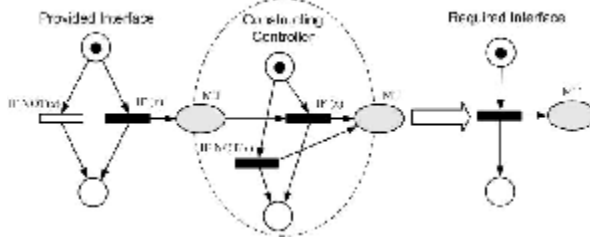
(a) Extra condition of sending messages scenario
