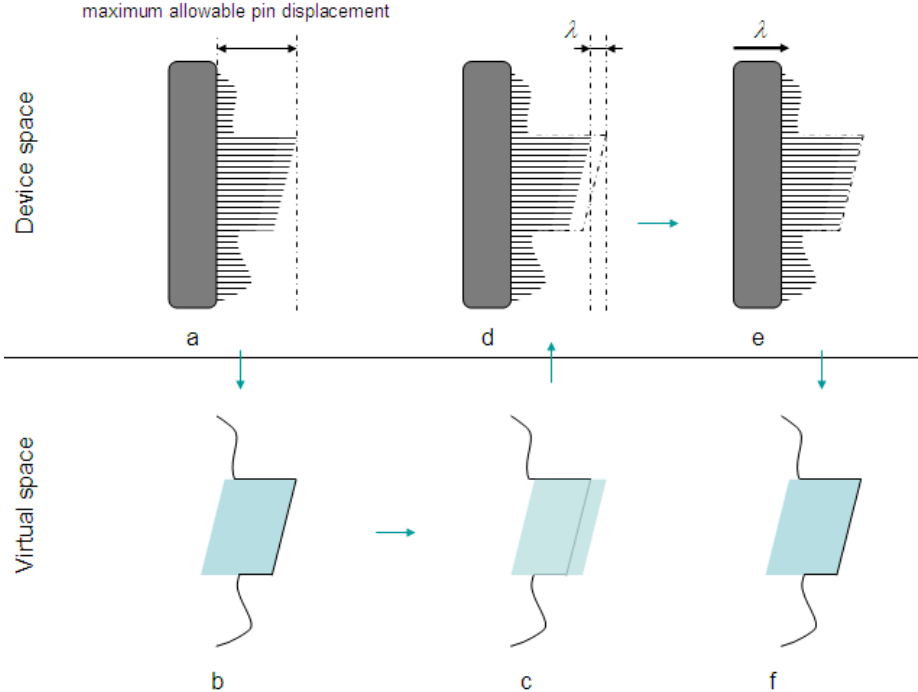
Figure 4. Example of robot motion. When the virtual object creates a displacement greater than can be absorbed by the pin range, the robot arm moves the entire pin assembly. In the case above, the virtual object is moving the hand.
