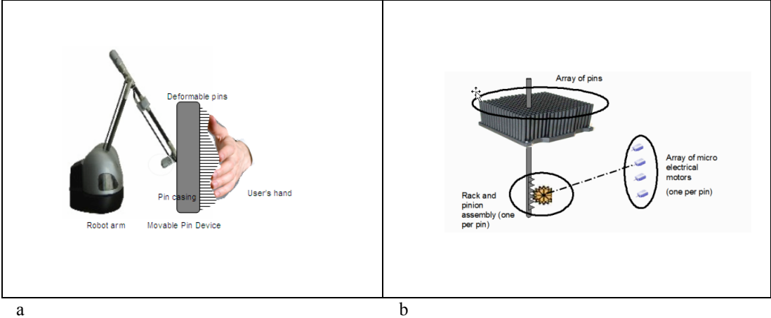
Figure 1. The controller for the virtual hand is an array of pins attached to a robot arm, shown in Panel a. The displacement of the pins represents the shape and texture of the objects in the virtual world. The 6 degree-of-freedom robot arm is based on previous art [3] . Panel b shows how pin displacement is controlled by an array of micro-electrical motors, one per pin, each driven by a rack and pinion assembly. The array of micro actuators acts as an output device, communicating properties of the virtual world to the user through pin displacements. It also serves as an input device, allowing the user to edit and transform the virtual world model by pressing on the pins.
