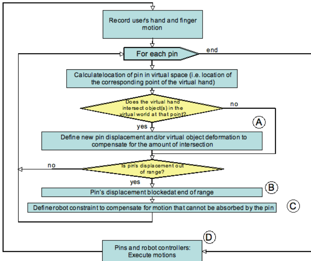
Figure 2. Control program that monitors pin displacement and adjusts the pin and robot controllers to execute appropriate motions to enable the movement of the virtual hand through the virtual space, allowing it to transducer the presence of surfaces and their textures, to edit these surfaces and textures, and to move objects in the space.
