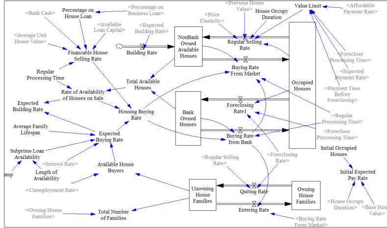
Figure 4: System Dynamics model for House Market
