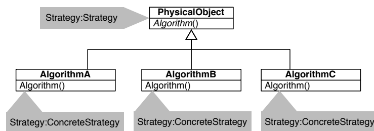
Figure 1: Pattern:role Annotation tags in UML
