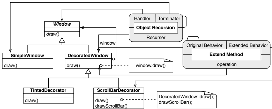
Figure 11: Peeled PIN instance used with UML
