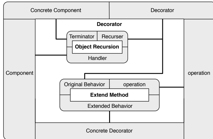
Figure 8: PIN Diagram of Design Pattern Definition
