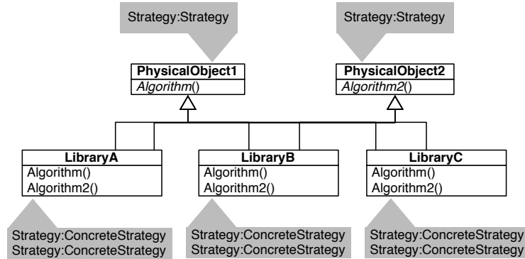
Figure 2: Pattern:role Annotation tags in UML - multiple instances
