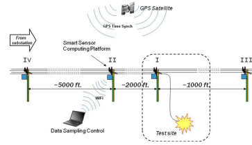
Fig. 2. Experiment setup.
