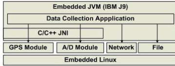
Fig. 3. Data Collection Application.
