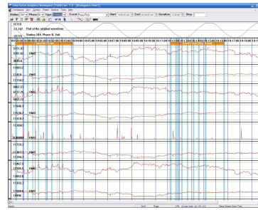
Fig. 4. Current and voltage waveforms recorded on Phase B at stations 101, 102, 104 and 104 respectively (top to bottom).
