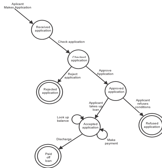
Figure 4. Life Cycle Diagram [Hawryskiewicz, 1988]
