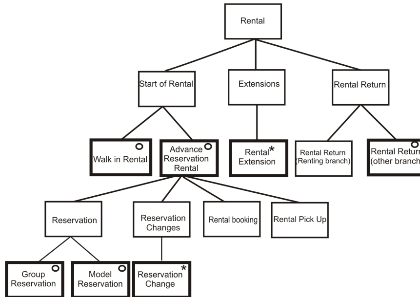
Figure 9. An example of entity-action diagram in Jackson's tradition and notation. In this diagram, the circle symbol in a box means selection (i.e., option) and the star means repetition.
