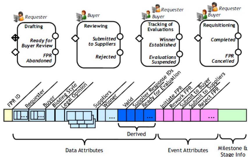
Figure 8 A Business Entity lifecycle using the GSM notation [Hull et al, 2010]
