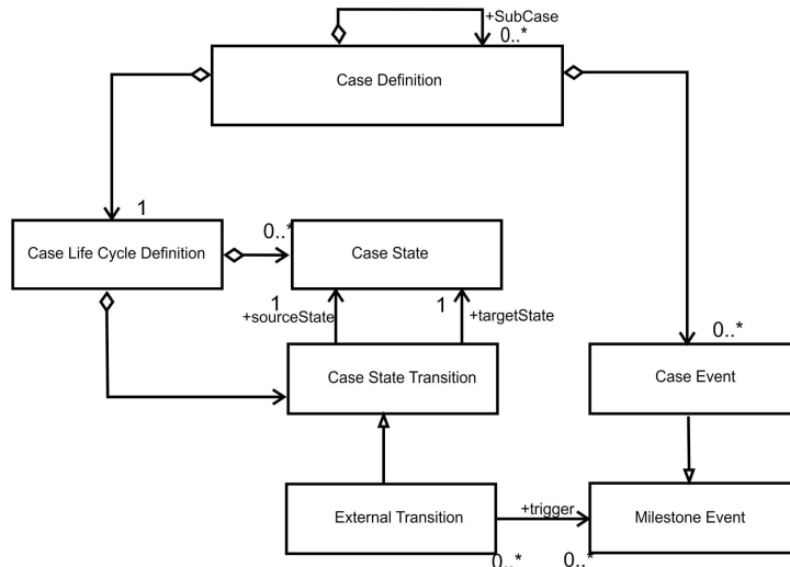
Figure 13. Case metamodel slightly adapted from [Cordys, on-line presentation] 26
