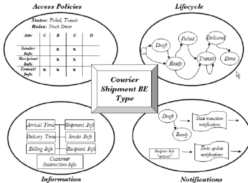
Figure 6. A diagram from Nandi et al [Nandi et al, 2010] showing an entity called “Courier Shipment”
