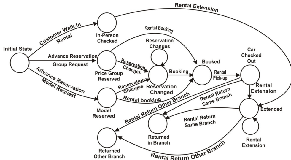
Figure 10. State Life Cycle equivalent representation of Figure 9 by following [Rosenquist, 1982], [Hawryszkiewicz, 1988], [Martin, 1990]
