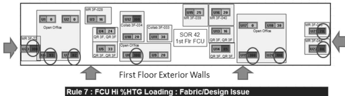
Fig 4 : Spatial Representation of Possible Fabric/FCU Design Capacity Problem
