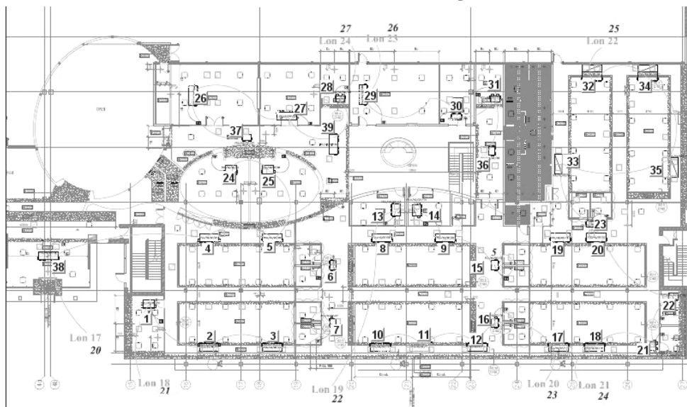
Fig 1 : Ground Floor Fan Coil Unit Spatial Floor Plan : U1 to U33
