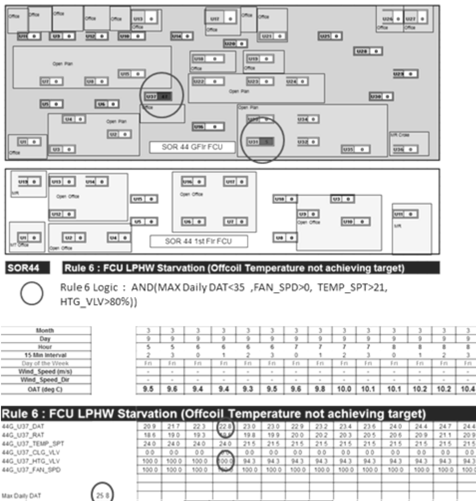
Fig 3 : Spatial Representation of Possible LPHW Strainer Problem
