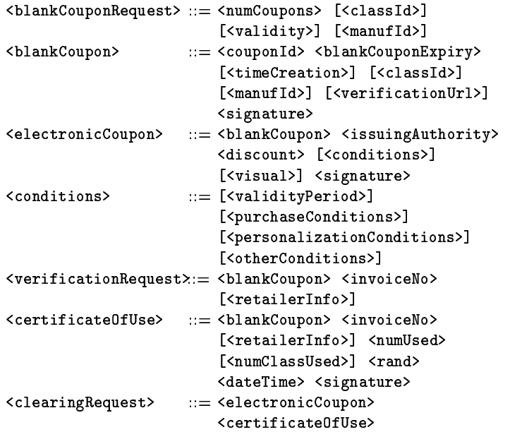
Figure 2: Messages exchanged in the electronic coupon system. The terms enclosed in [] are optional.
