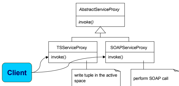
Figure 8. TSSAPI service proxies
