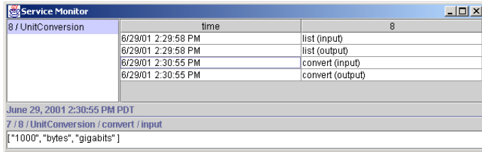
Figure 13. Using the Service Monitor to view a list of input and output messages
