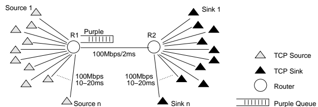
Fig. 1. Simulation topology for the single-bottleneck case.
