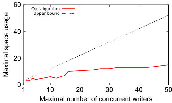
Figure 4: The maximal space usage depending on the number of concurrent writers. The upper bound is the number of writers plus two according to Theorem 9.
