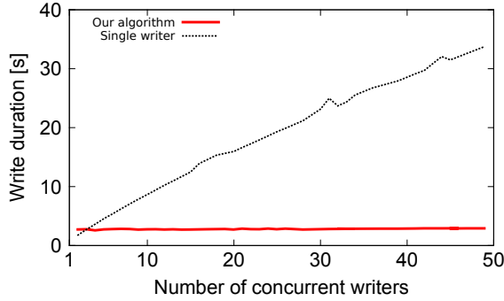
Figure 3: The average duration of write operations as a function of the number of concurrent writers. The single-writer approach with serialized operations is shown for comparison.
