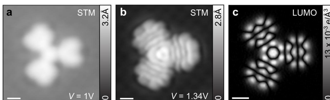
Figure 2. Constant-current STM measurements (tunnel current I = 2 pA, T = 5 K) of trimer 1 on NaCl(2ML)/Cu(111) using a CO tip. Measurements were acquired at sample voltages of V = 1.0 V, i.e., in the gap below the onset of the LUMO in a), and at V = 1.34 V, i.e., at the onset of the LUMO in b). In c) the calculated orbital density squared of the LUMO at a distance of 1.2 Å above the molecular plane is shown. The scale bars are 5 Å.
