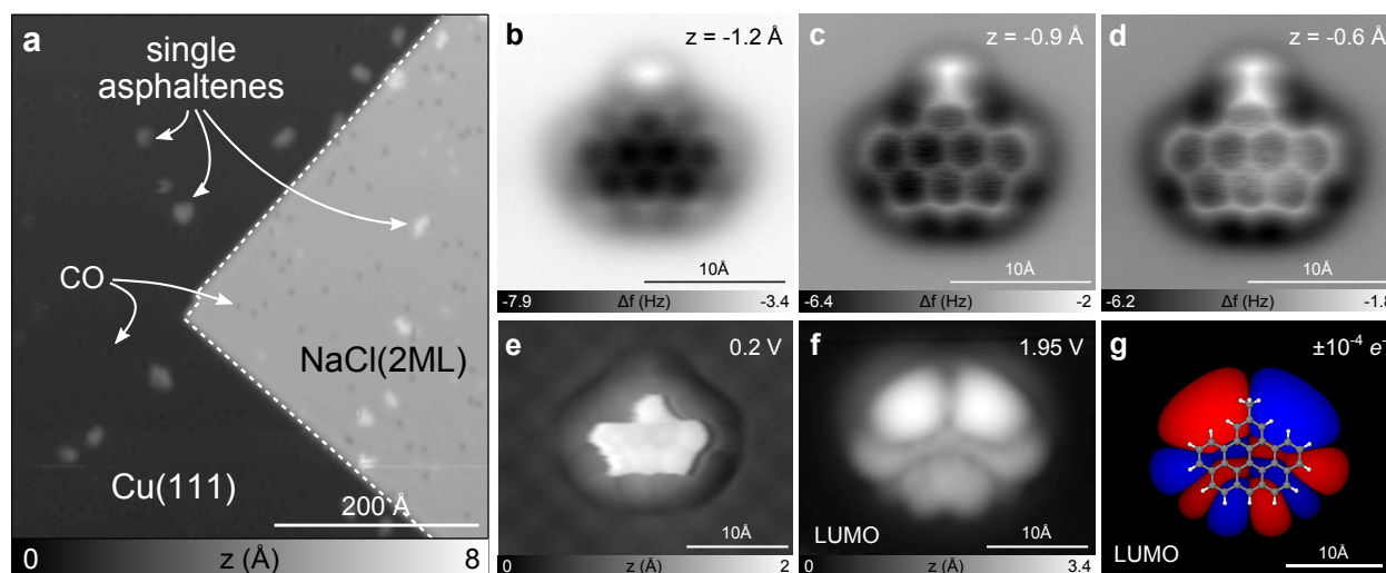
Figure 1: Coal-derived asphaltene sample preparation and CA1. a STM overview image ( I = 1 pA, V = 0.5 V) of the CA sample on NaCl(2ML)/Cu(111). b-d AFM images of CA1 on NaCl(2ML)/Cu(111) at different set-points z from ( I = 1.4 pA, V = 0.2 V). e STM image of CA1 ( I = 10 pA, V = 0.2 V). f STM image at the NIR ( I = 1.4 pA, V = 1.95 V). g LUMO orbital of CA1 with the molecular structure overlaid as a guide to the eye. CO-functionalized tips have been used for all AFM and STM measurements shown.
