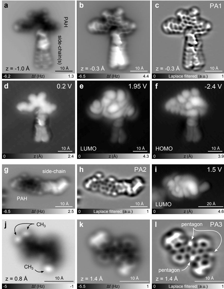
Figure 5: Petroleum asphaltenes PA1-PA3. a,b AFM images of PA1 on NaCl(2ML)/Cu(111) at different set-points z from ( I = 1 pA, V = 0.2 V). c Laplace-filtered image of b . d-f STM images ( I = 1 pA) of PA1 recorded at 0.2 V, 1.95 V and -2.4 V, respectively. g,h AFM image of PA2 on NaCl(2ML)/Cu(111) ( g ) and its Laplace-filtered version ( h ). i STM orbital image ( I = 0.6 pA) of PA2 corresponding to the LUMO resonance. On the left side of g-i there is a small patch of third-layer NaCl. j,k AFM images of PA3 on NaCl(2ML)/Cu(111) at different set-points z from ( I = 1.8 pA, V = 0.2 V). l Laplace-filtered image of k .
