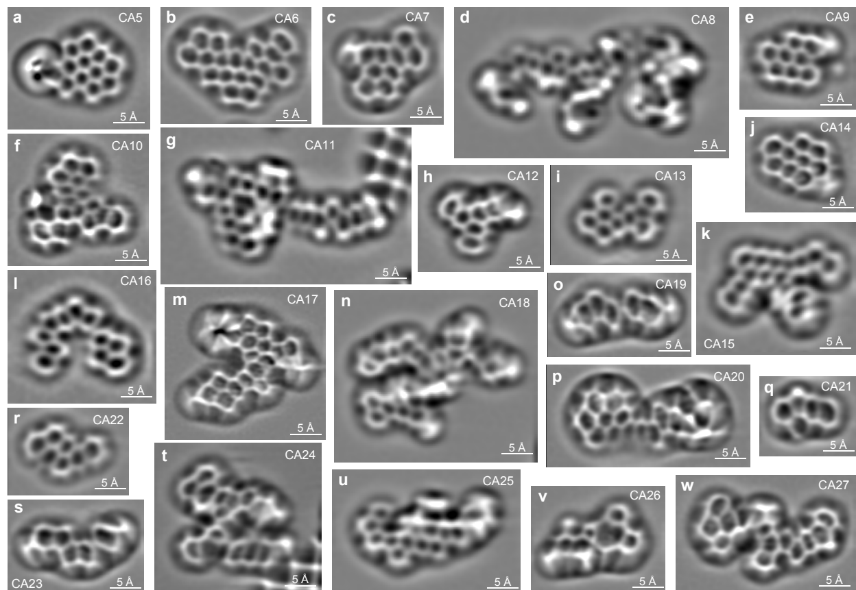
Figure 3: Coal-derived asphaltenes CA5-CA27. a-w Laplace-filtered AFM images of different CAs on Cu(111) or NaCl(2ML)/Cu(111). In g and t , a small patch of third-layer NaCl is also imaged. The AFM raw data and orbital images for some molecules are available in Fig. S1 and Fig. S2, respectively.
